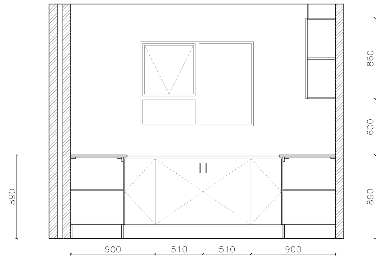
Kitchen Elevation C
