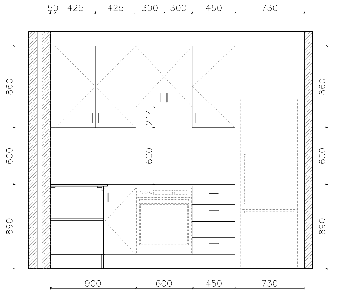
Kitchen Elevation B
