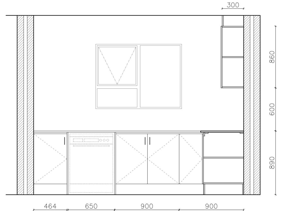
Kitchen Elevation A
